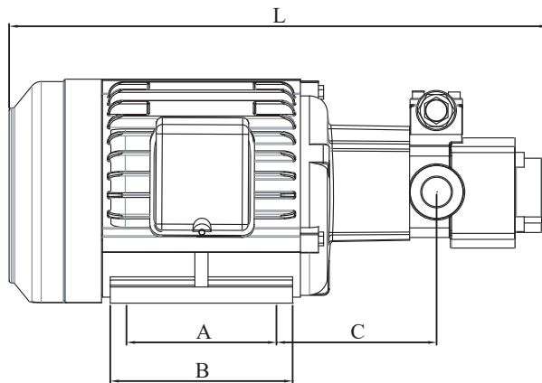
RBB-22 帶聯軸器電機組尺寸圖表 (WITH COUPLING)
