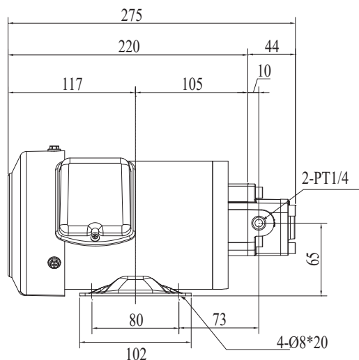
RBB-2帶聯軸器電機組尺寸圖表 (WITH COUPLING)
