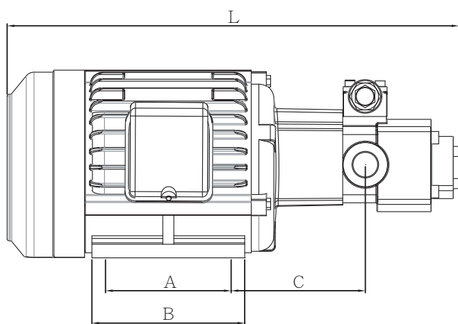
RBB-2帶聯軸器電機組尺寸圖表 (WITH COUPLING)
